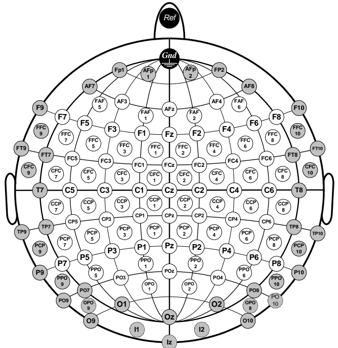
Figure 3: Locations of electrodes and labels of corresponding channels.
