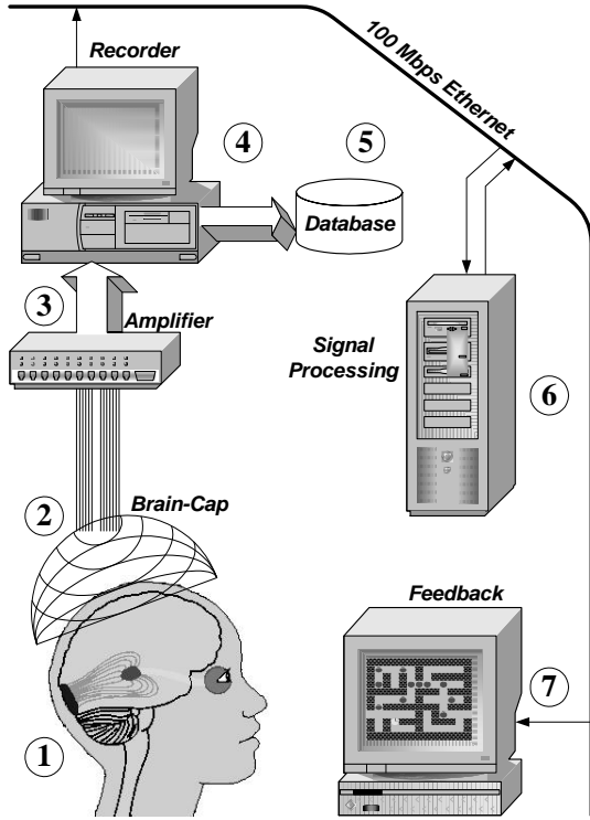
Figure 1: Distributed design of BBCI.
