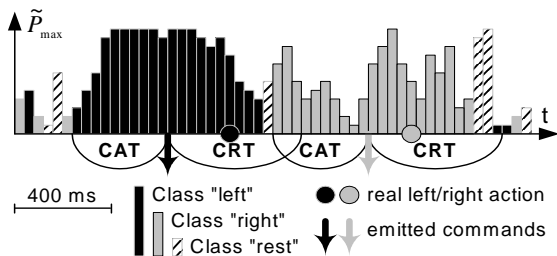
Figure 8: Time structure of command emission queue
