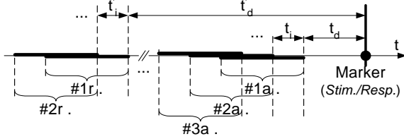
Figure 6: Selection procedure for training samples
