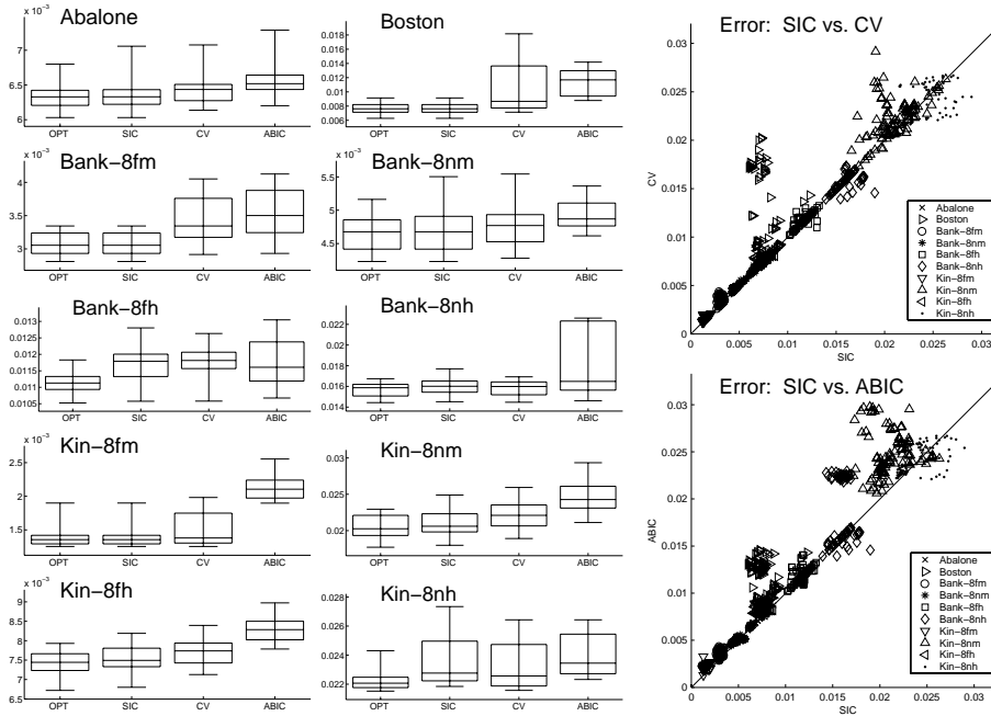
Fig. 2. Simulation results with DELVE data sets (Gaussian kernel).
