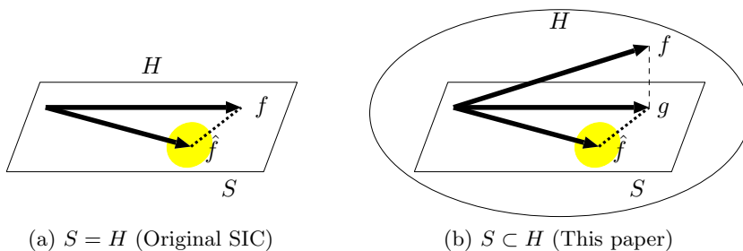
Fig. 1. Original SIC and extension carried out in this paper. H is a reproducing kernel Hilbert space that includes the learning target function f . S is the subspace spanned by \{k(\mathbf{x}, \mathbf{x}_m)\}_{m=1}^M . g is the orthogonal projection of f onto S . (a) Setting of the original SIC [5]. It was shown that when S = H , SIC is an unbiased estimator of the generalization error between \hat{f} and f with finite samples. S = H implies that the RKHS H whose dimension is at most M ( < \infty ) is considered. (b) Setting of this paper. We consider the case that S \subset H , which allows any RKHS H including infinite dimensional ones. We show that the extended SIC is an unbiased estimator of the generalization error between \hat{f} and g .
