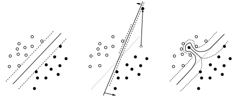
Fig. 2. The problem of finding a maximum margin “hyper-plane” on reliable data (left), data with an outlier (middle) and with a mislabeled pattern (right). The solid line shows the resulting decision line, whereas the dashed line marks the margin area. In the middle and on the right the original decision line is plotted with dots. Illustrated is the noise sensitivity: only one strong noise/outlier pattern can spoil the whole estimation of the decision line. From [23].
