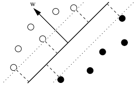
Fig. 1. Linear classifier and margins: A linear classifier is defined by a hyperplane's normal vector \mathbf{w} and an offset b , i.e. the decision boundary is \{\mathbf{x} | \mathbf{w}^\top \mathbf{x} + b = 0\} (thick line). Each of the two halfspaces defined by this hyperplane corresponds to one class, i.e. f(\mathbf{x}) = \text{sign}(\mathbf{w}^\top \mathbf{x} + b) . The margin of a linear classifier is the minimal distance of any training point to the hyperplane. In this case it is the distance between the dotted lines and the thick line. From [9].
