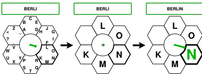
Fig. 5. The mental typewriter "Hex-o-Spell". The two states of the BCI system control rotation and extension of the arrow. After selecting a group of letters, a single letter can be chosen by selecting the hexagonal field containing the letter. See text for details.
