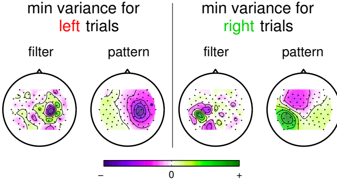
Fig. 2. The common spatial pattern (CSP) algorithm determines spatial structures which represent the optimal discrimination between two classes with respect to variance. The patterns illustrate how the presumed sources project to the scalp. They can be used to verify neurophysiological plausibility. The filters are used to project the original signals. They resemble the patterns but their intricate weighting is essential to obtain signals that are optimally discriminative with respect to variance. These two CSP filters were calculated from the calibration data of subject aa and have been used for feedback. Generally in this study 3 patterns/filters of each type were calculated. Neurophysiologically unplausible pattern/filter pairs were discarded from the use in online feedback.
