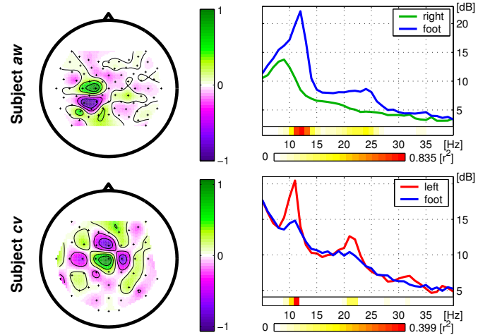
Fig. 4. Left: Scalp topographies for subjects aw and cv one of the selected CSP filters. Right: Spectra for the spatially filtered signals with color coded r^2 -values for the difference between the two classes below. These plots exemplarily show for two subjects that CSP filter improves the discriminability of the two conditions compared to the best Laplacian filtered channel substantially, cf. Fig. 3.
